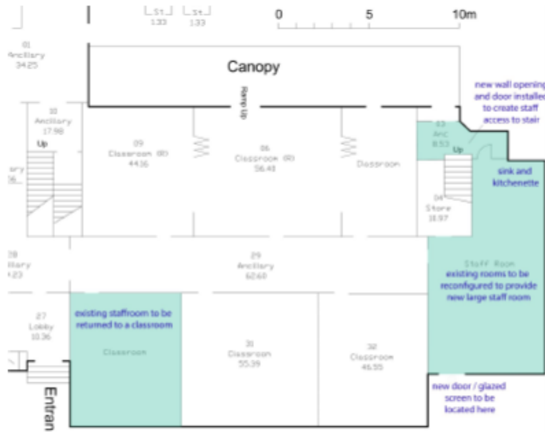
Fig 7 — Ground floor sketch plan (staff area)
