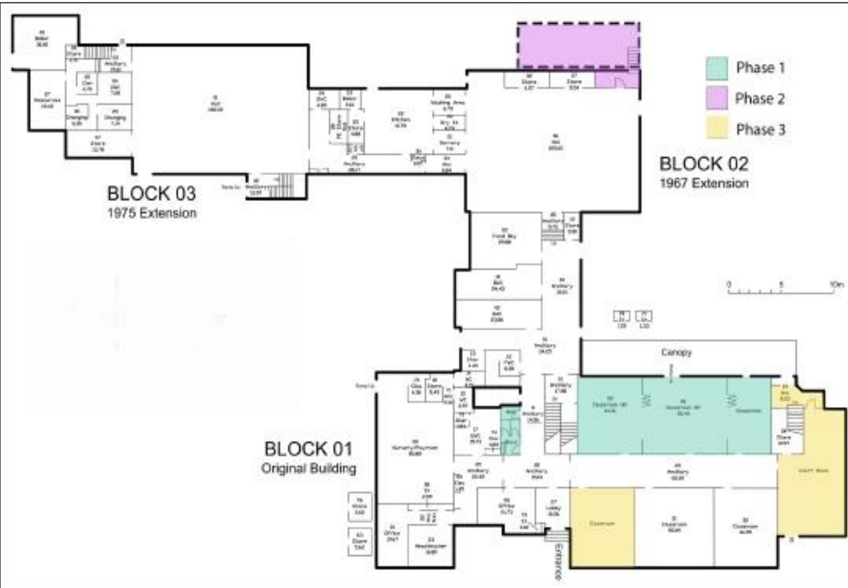
Fig 12 — Ground floor phasing plan
